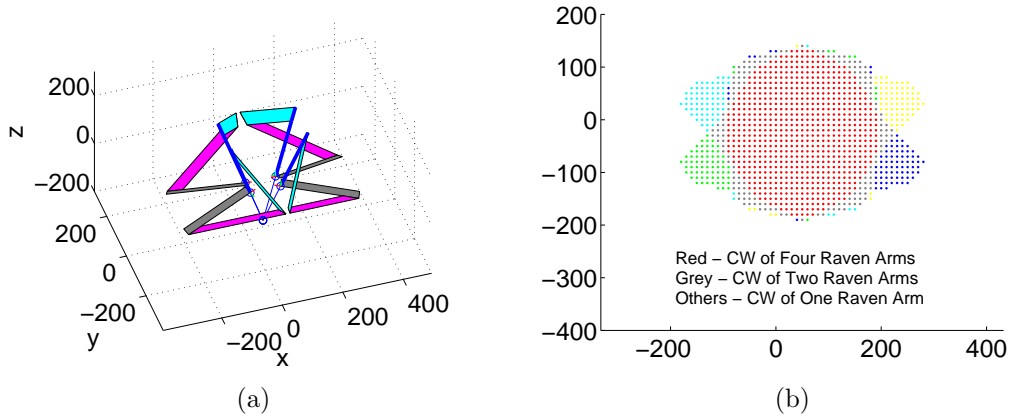
Figure 11.12: Optimal configuration of the Raven IV surgical robot four arms following a brute force search (a) Relative position and orientation of the system bases (b) optimized workspace.
