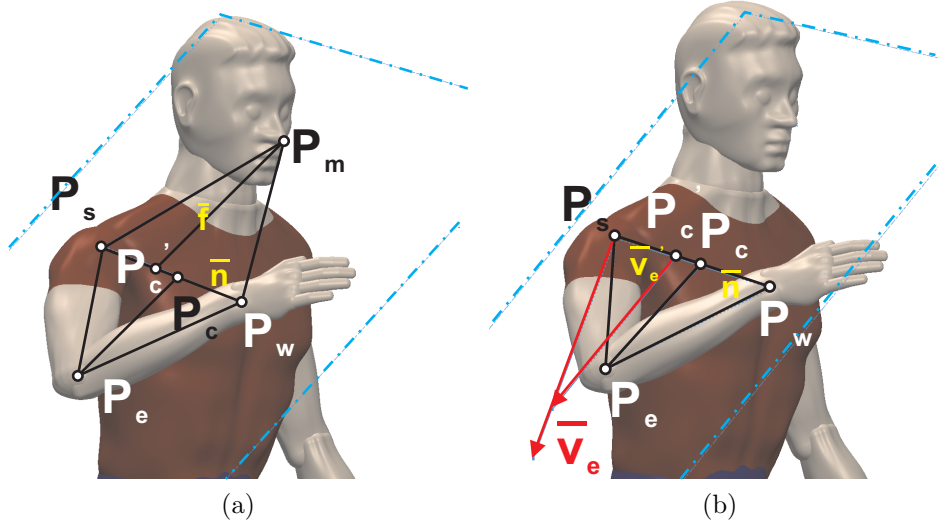
Figure 4.3: (a) Criterion 1 maximizes motion efficiency by maximizing the projection of the longest principle eigen-vector of the manipulability ellipsoid on the direction from the hand to the virtual target P_m . The corresponding elbow position falls on the plane formed by P_s , P_w and P_m . (b) Criterion 2 intends to maintain the arm posture close to the equilibrium arm posture by placing the elbow on the plane formed by the wrist position P_w and the direction of the equilibrium vector \vec{v}_e .
