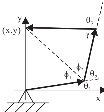
Figure 10.6: Family 1: \theta_1 > 0, \theta_2 > 0, \theta_3 > 0 .
