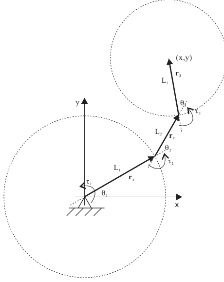
Figure 10.3: Three-link mechanism.
