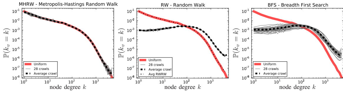
Fig. 5. Degree distribution (pdf) estimated by the sampling techniques and the ground truth (uniform sampler). MHRW and RWRW agree almost perfectly with the UNI sample; while BFS and RW deviate significantly.
