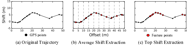
Figure 11: Examples of Trajectory Feature Extraction
