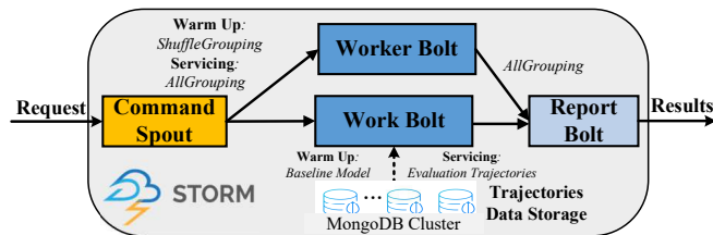
Figure 13: Cloud-based Deployment.
