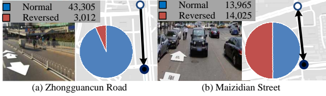
Figure 9: Results of Reverse Trajectory Identification.
