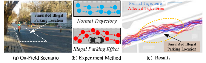
Figure 3: Intuition Validation Experiments.
