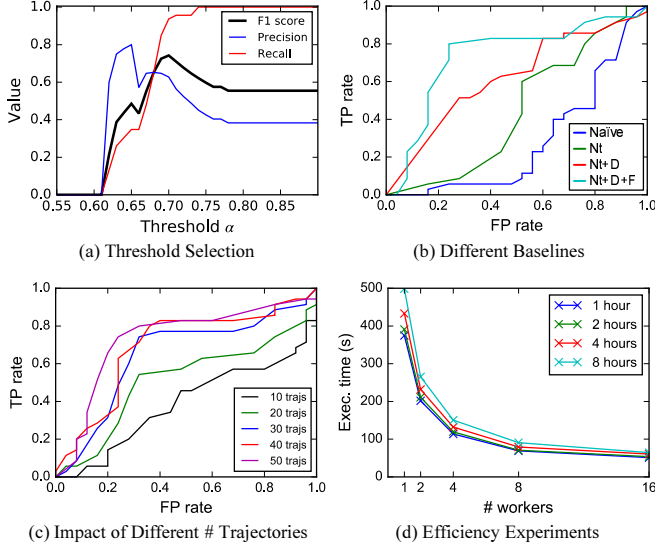
Figure 14: Effectiveness & Efficiency Experiments.
