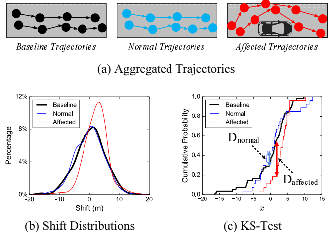
Figure 10: Main Ideas of Illegal Parking Detection.
