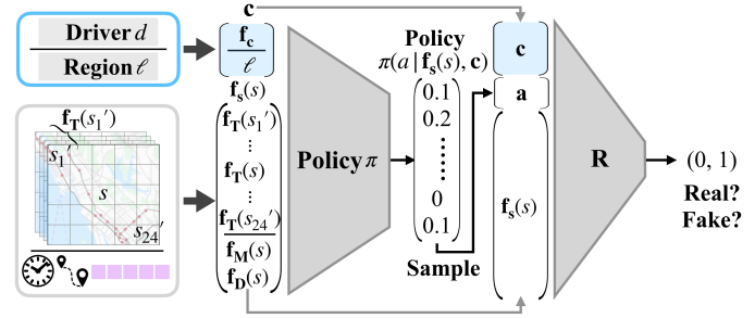
Fig. 4: cGAIL model structure.
