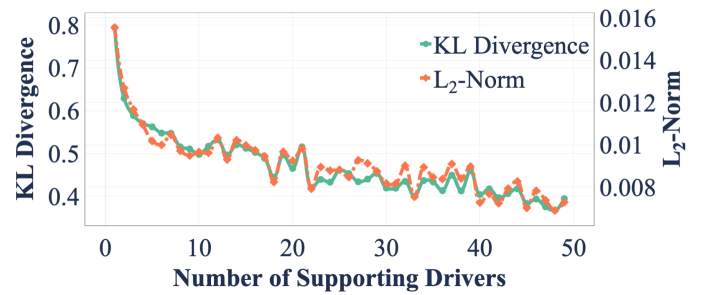
Fig. 10: Number of supporting drivers.
