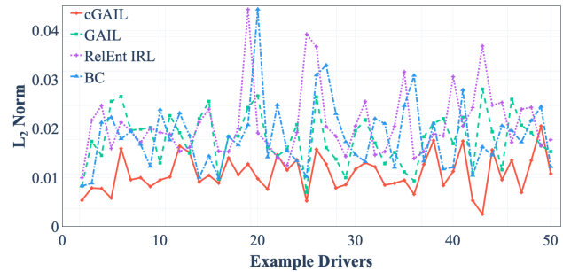
Fig. 5: Comparison with baselines
