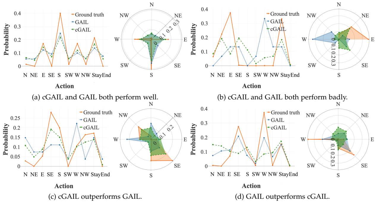
Fig. 11: cGAIL and GAIL performance case studies.
