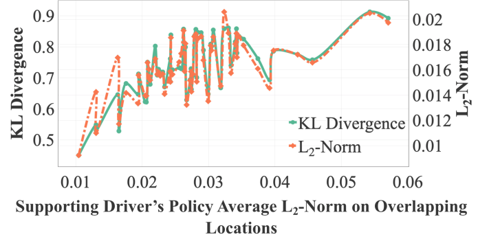
(c) Policy similarity in L_2 -norm. Fig. 9: Effects of cGAIL parameters.
