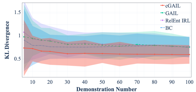
Fig. 7: KL divergence and standard deviation change with cold spot demonstration number.
