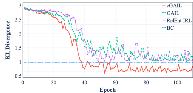
Fig. 6: Learning curves of cGAIL, GAIL and RelEnt IRL.
