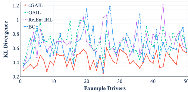
Fig. 5: Comparison with baselines
