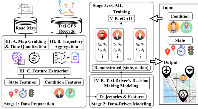
Fig. 2: Solution Framework.
