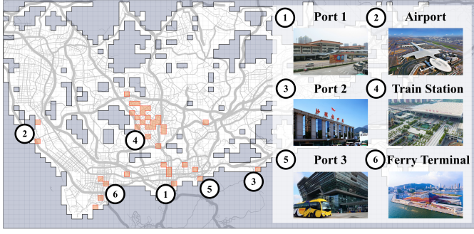
Fig. 8: 20 testing locations of an example driver agent. data was collected for d at \ell , cGAIL can still accurately estimate d 's policy at \ell by transferring knowledge from other “supporting” drivers used in the training process. However, given a target driver d , data from different supporting drivers may have diverse abilities to assist learning the policy of d at a location \ell . Intuitively, the more “similar” the supporting drivers are to the target driver, the more knowledge we can utilize to “support” learning the policy of target driver d . Below, we evaluate how two similarity measures between the target and supporting drivers and the total number of supporting drivers affect the accuracy of learned policy for target drivers at various locations. We run our experiments over all expert drivers (as target drivers separately) in the selected group \mathcal{E} . Similar results were obtained for all drivers, where we demonstrate the results from a few example drivers. Fig. 8 illustrates one example target driver, with orange grid cells as 20 testing locations selected with the number of visits more than 2,000 times. Clearly, those highly visited locations are primarily transport stations, airport, as marked in the figure. In the training process, we hide the data from the 20 testing locations to train cGAIL, and compare the difference between the learned policies and the true policies observed in the data.
