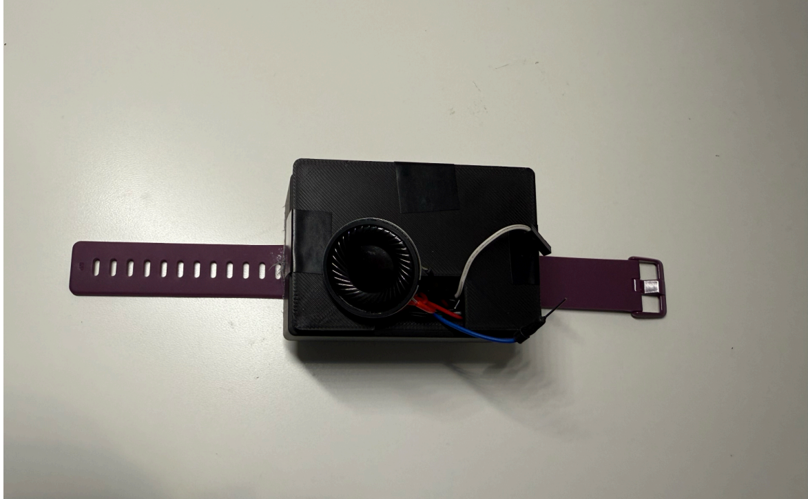
Figure 1: Image of the wrist wearable device with the lid attached, and the speaker extruding through the hole on the lid to be able to provide users with sensory feedback.
