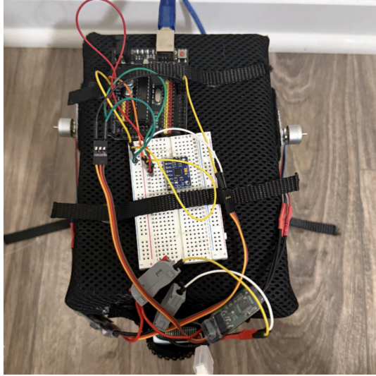
Figure 3: Bird's-eye view of device on mass-spring system
