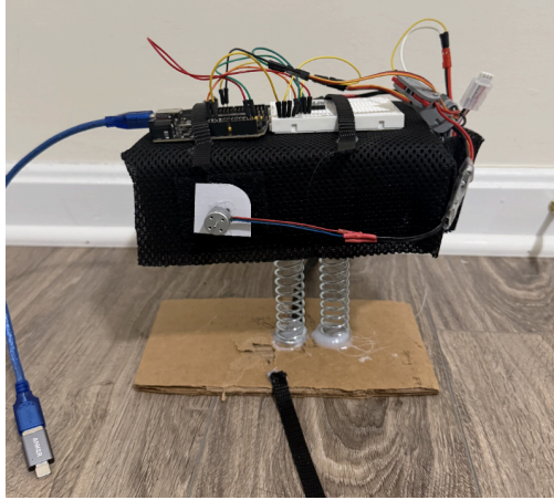
Figure 4: Side view of device on mass-spring system
