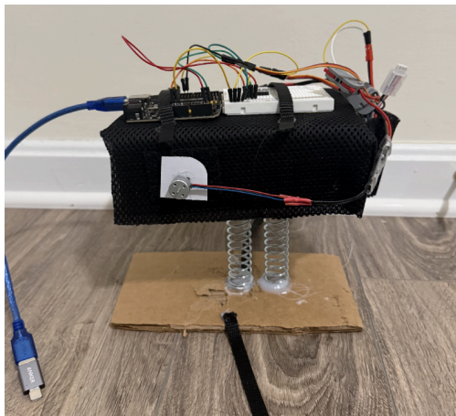
Figure 2: Side view of device on mass-spring system
