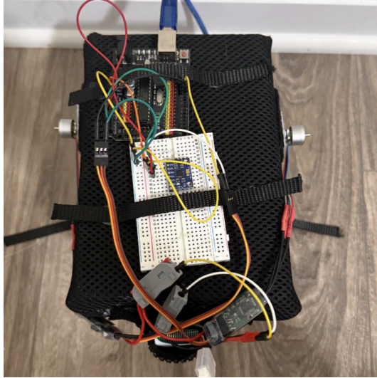
Figure 1: Bird's-eye view of device on mass-spring system
