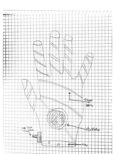
Figure 4. Design 4: copper wires (MR signalling) wrap around flexible glove. MR fluid is taken in and replaced through valve (left). System is fully sealed with small ventilation valve for comfort (Golji et al., 2026).
