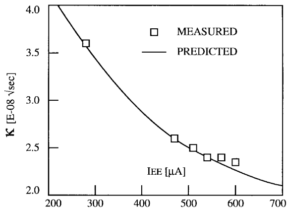
Fig. 6. \kappa versus tail current IEE.
