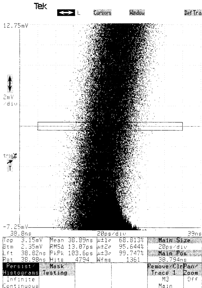
Fig. 7. Measured closed-loop jitter of 622 MHz PLL.
