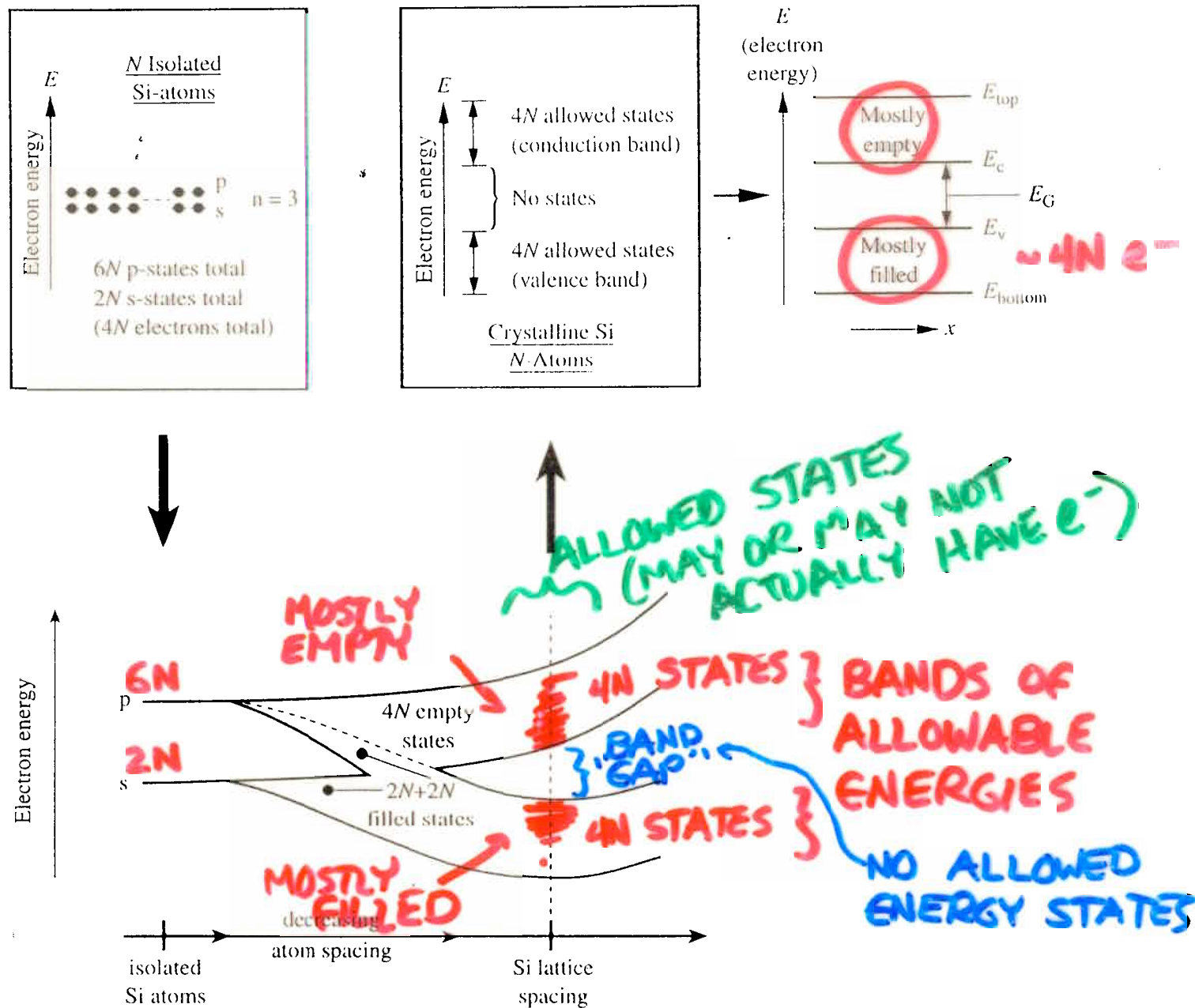
Figure 2.5 Conceptual development of the energy band model starting with N isolated Si atoms on the top left and concluding with a “dressed-up” version of the energy band model on the top right.
