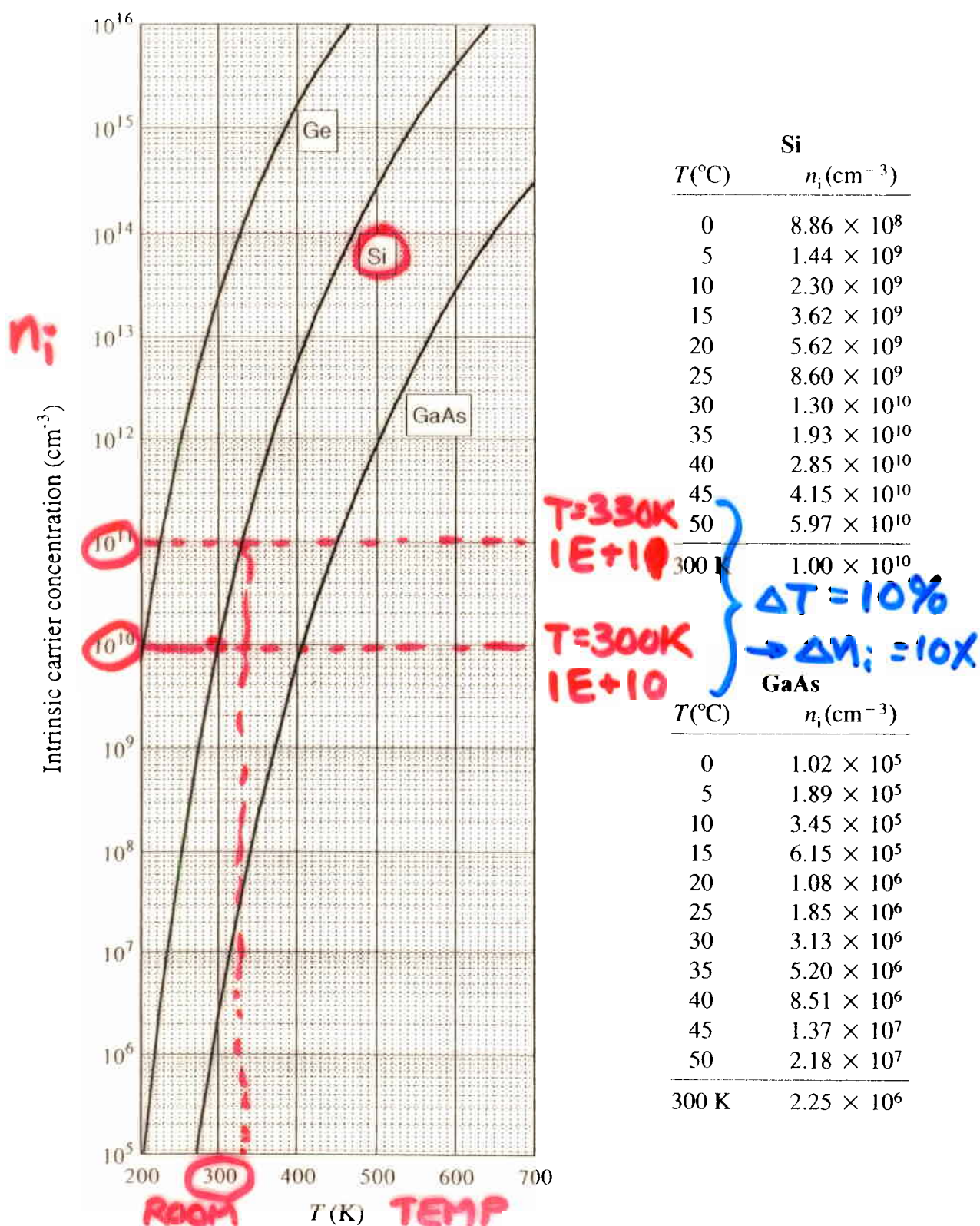
Figure 2.20 Intrinsic carrier concentrations in Ge, Si, and GaAs as a function of temperature.
