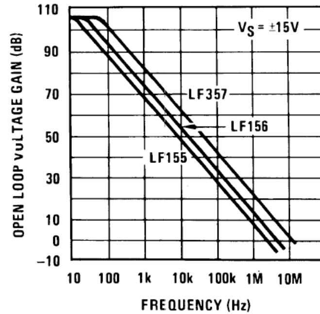
Open Loop Frequency Response
