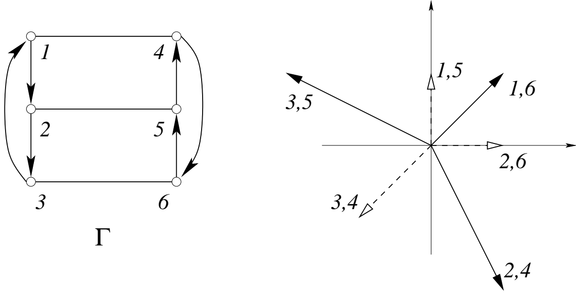
Figure 1: Eigenspace representation of \text{dsrg}(6, 2, 1, 0, 1) is not injective. Left representation y_j of a vertex j is solid while x_j is hollow/dashed.
