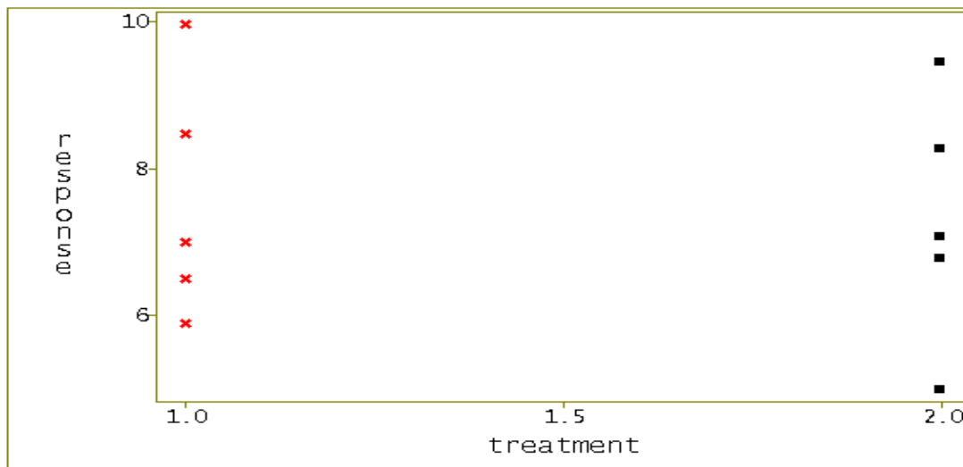
Figure 1: Scatter plot of fabricated data viewed as unpaired. Observations from treatment 1 are in red with an 'x' plotting symbol.
