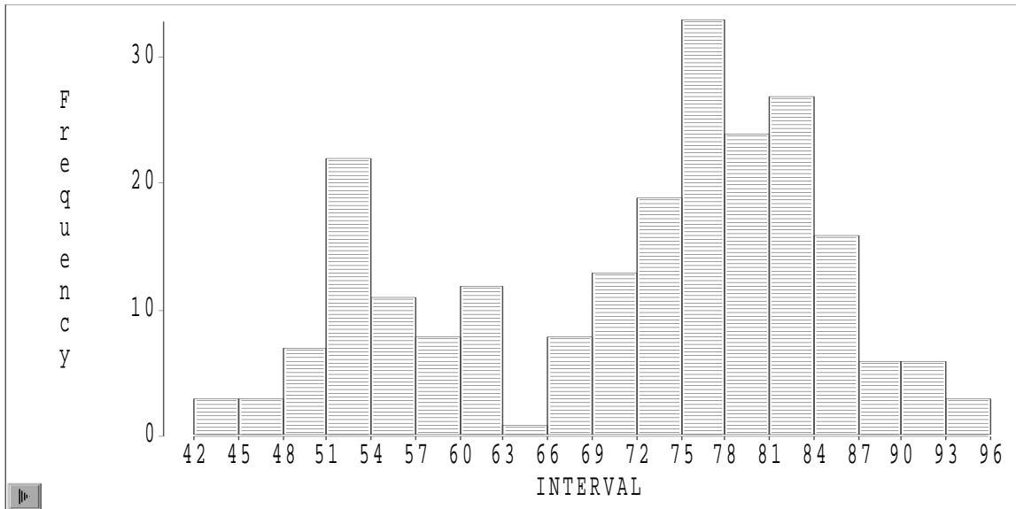
Figure 6: Frequency histogram of the intervals between eruptions of the Old Faithful geyser.
