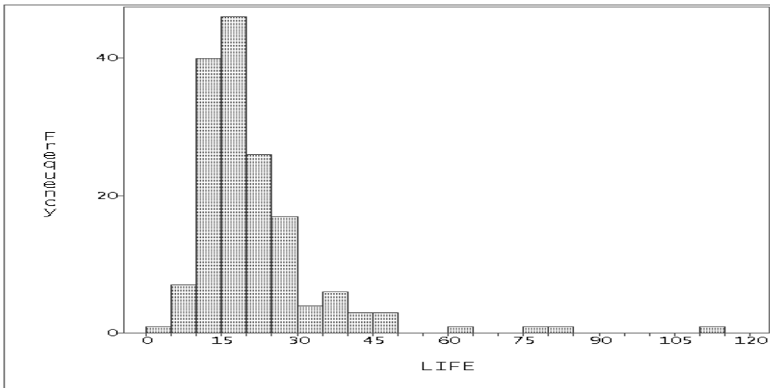
Figure 4: Frequency histogram of lifetimes of 157 electrical transformers.
