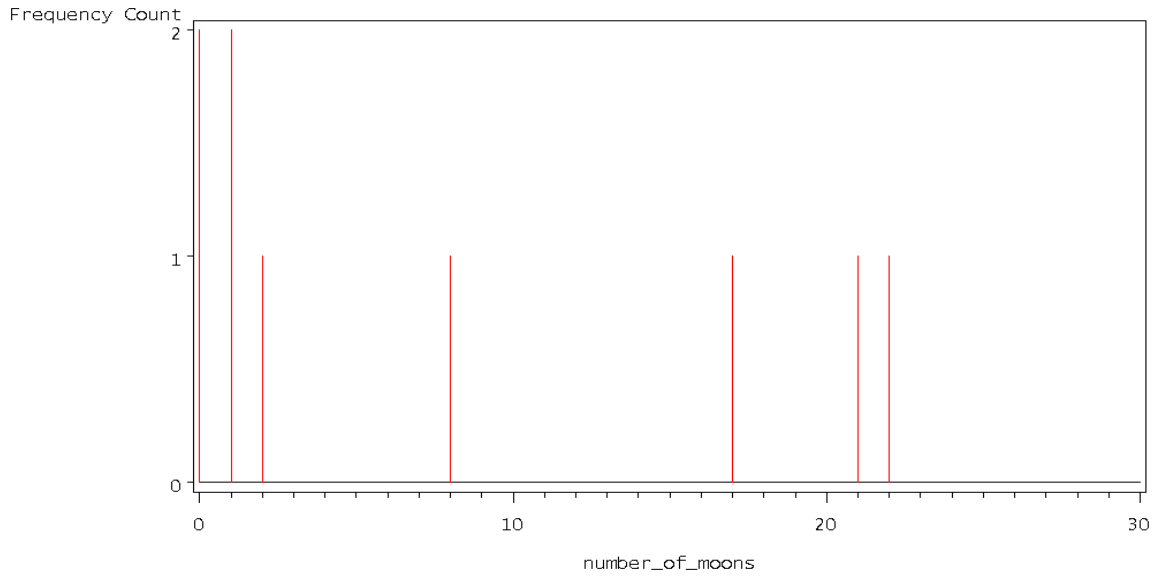
Figure 2: Needle plot of the numbers of moons among the nine planets.
