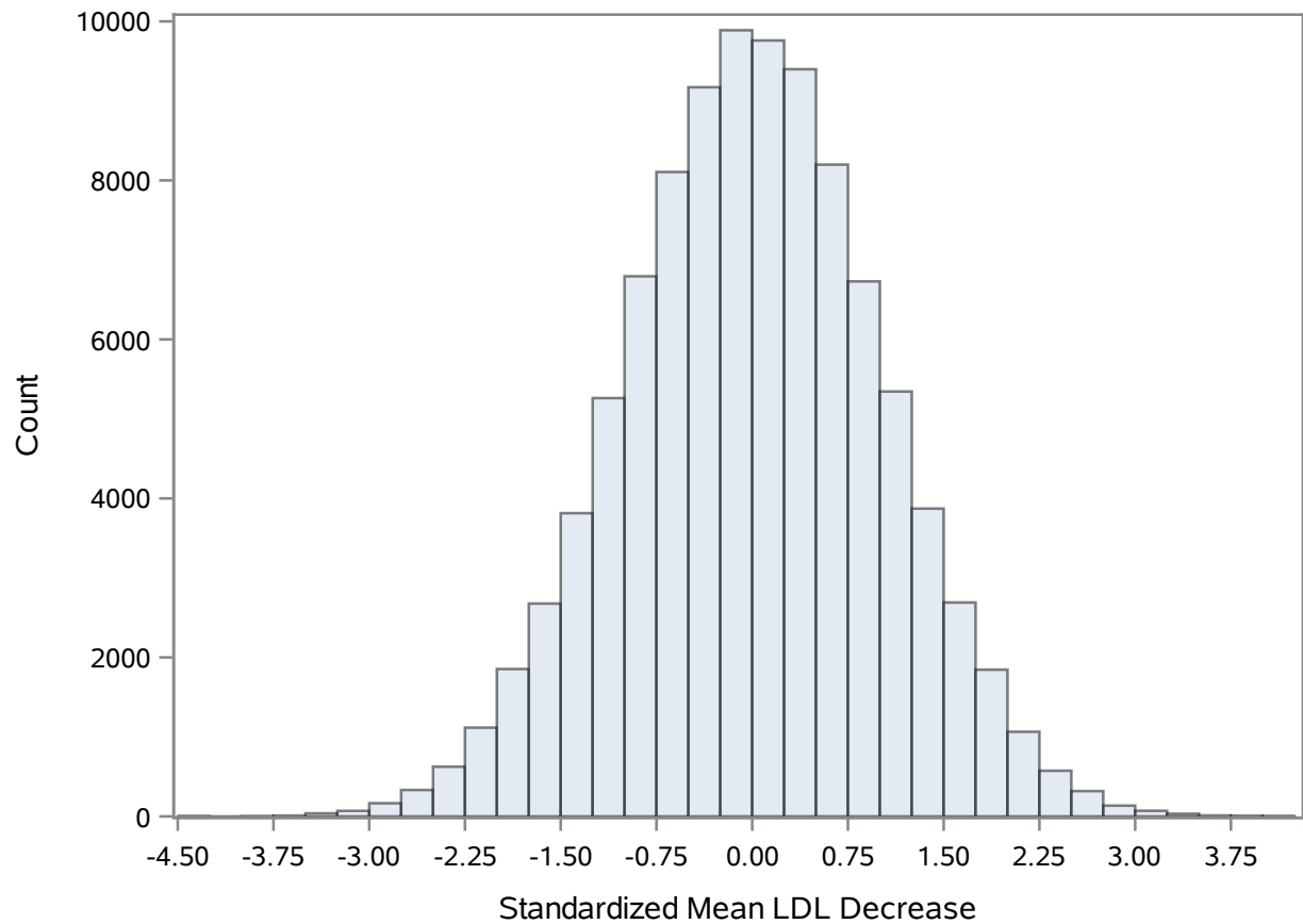
Distribution of y
