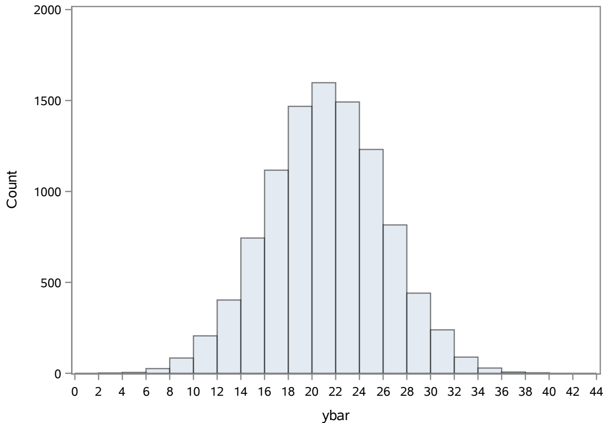
Distribution of ybar
