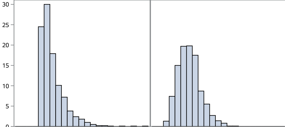
plot = Means of Size 30
