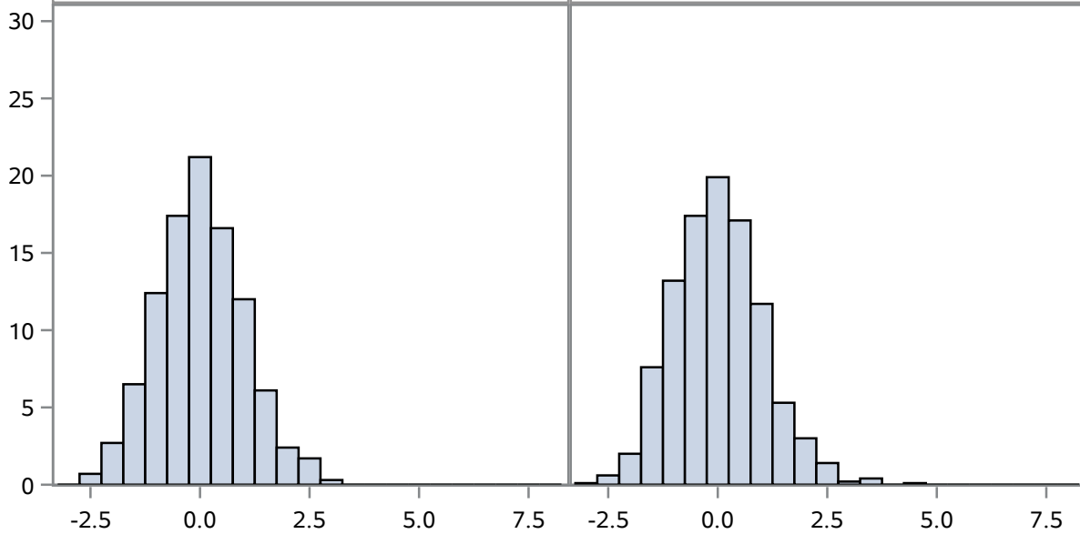
plot = Means of Size 30
