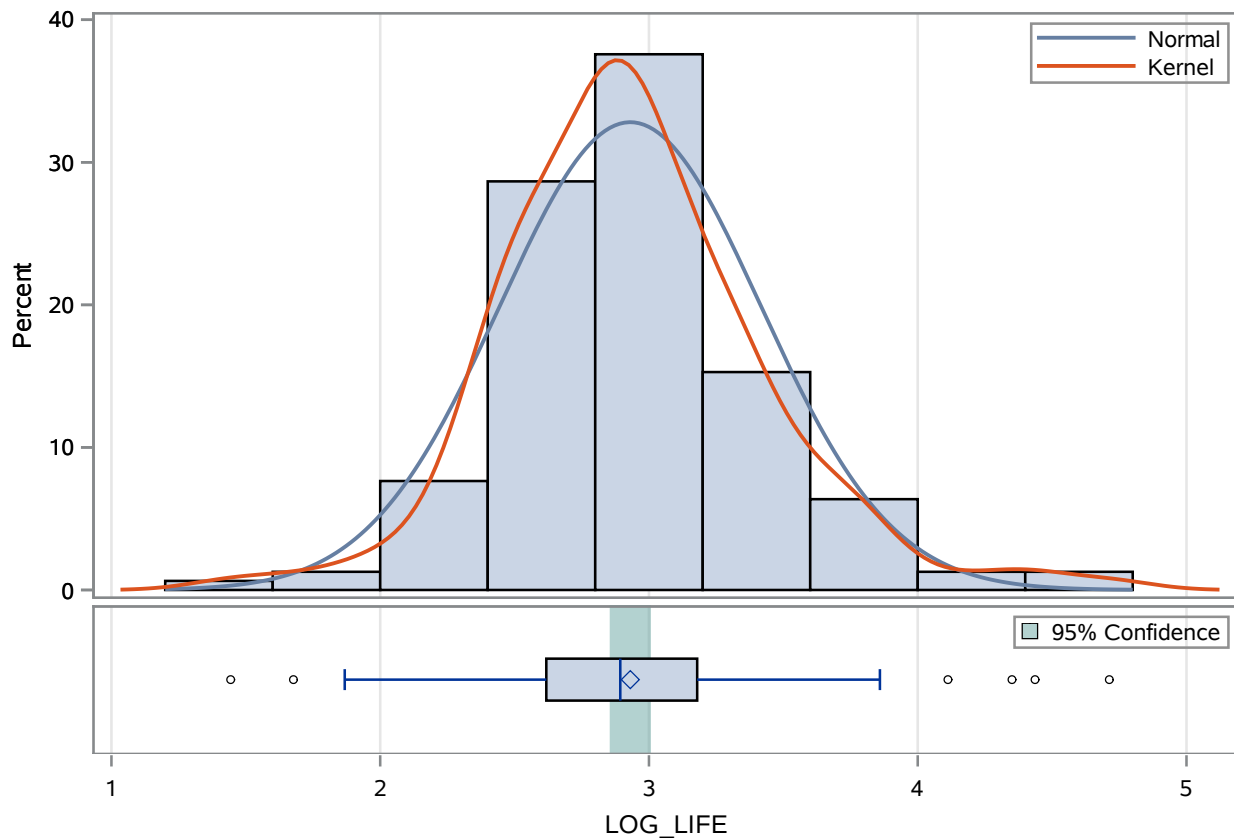
Distribution of LOG_LIFE With 95% Confidence Interval for Mean
