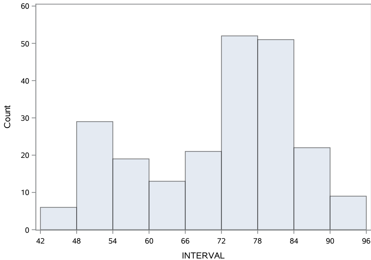
Distribution of INTERVAL
