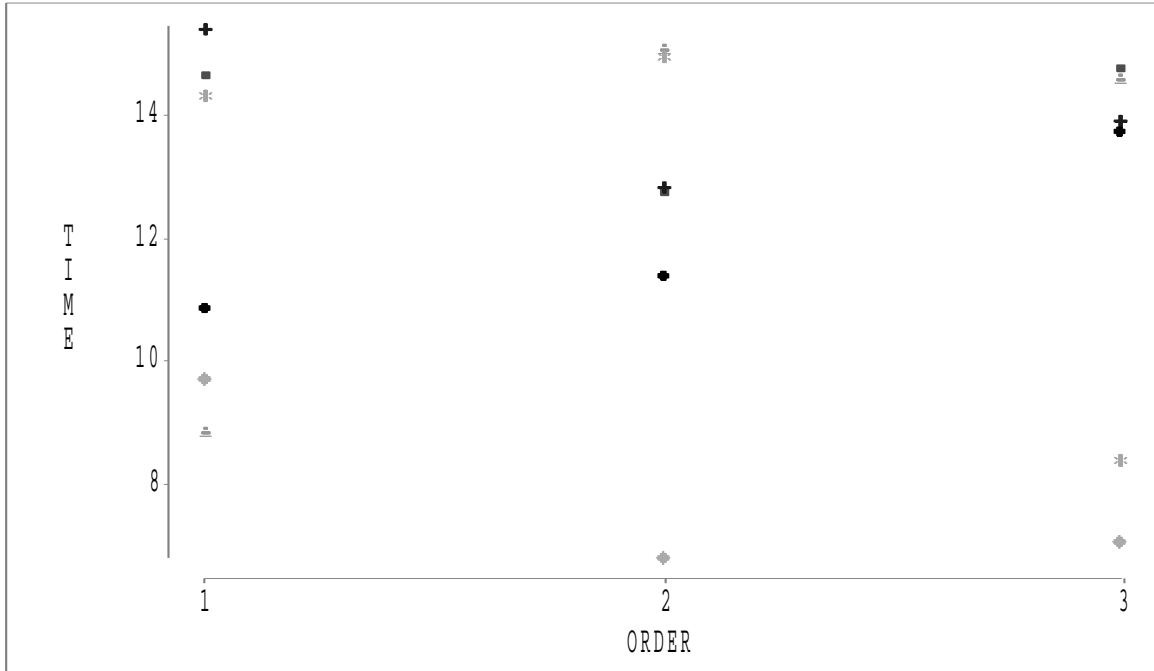
Figure 1: Funnel Data: Scatterplot of Time versus Order
