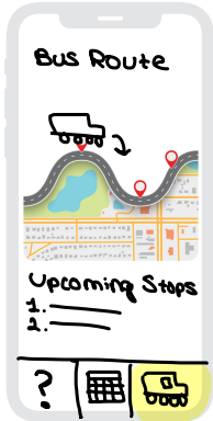
Bus Screen
