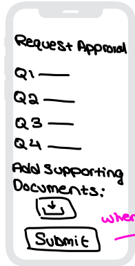
Approval Screen
