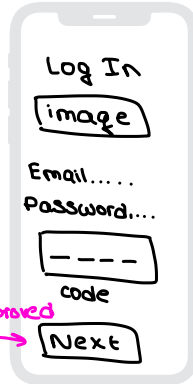
Grandp. login
