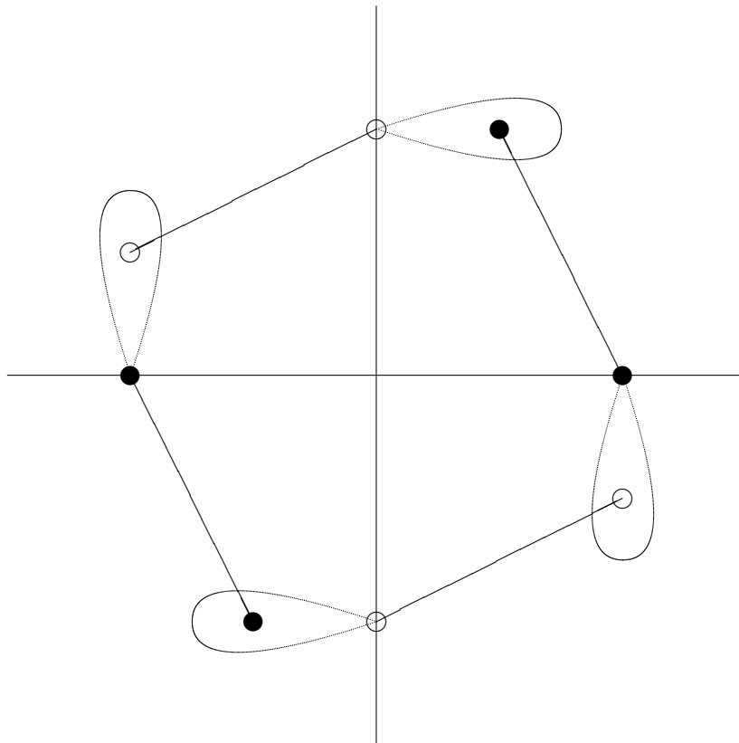
FIGURE 29. [2, 4^+] \triangleright [2, 2^+]
