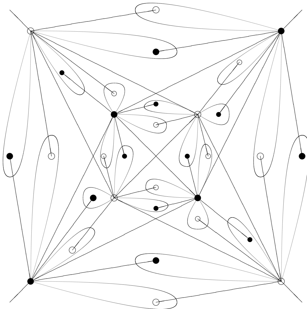
FIGURE 33. [3, 4]^+ \triangleright [3, 3]^+
