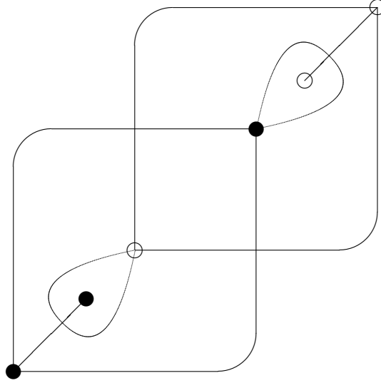
FIGURE 11. [2] \triangleright [1]
