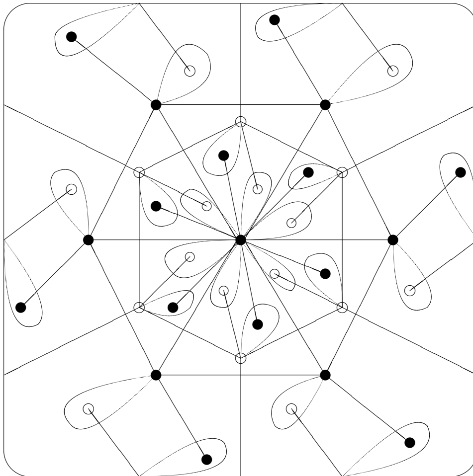
FIGURE 21. [2, 6]^+ \triangleright [6]^+
