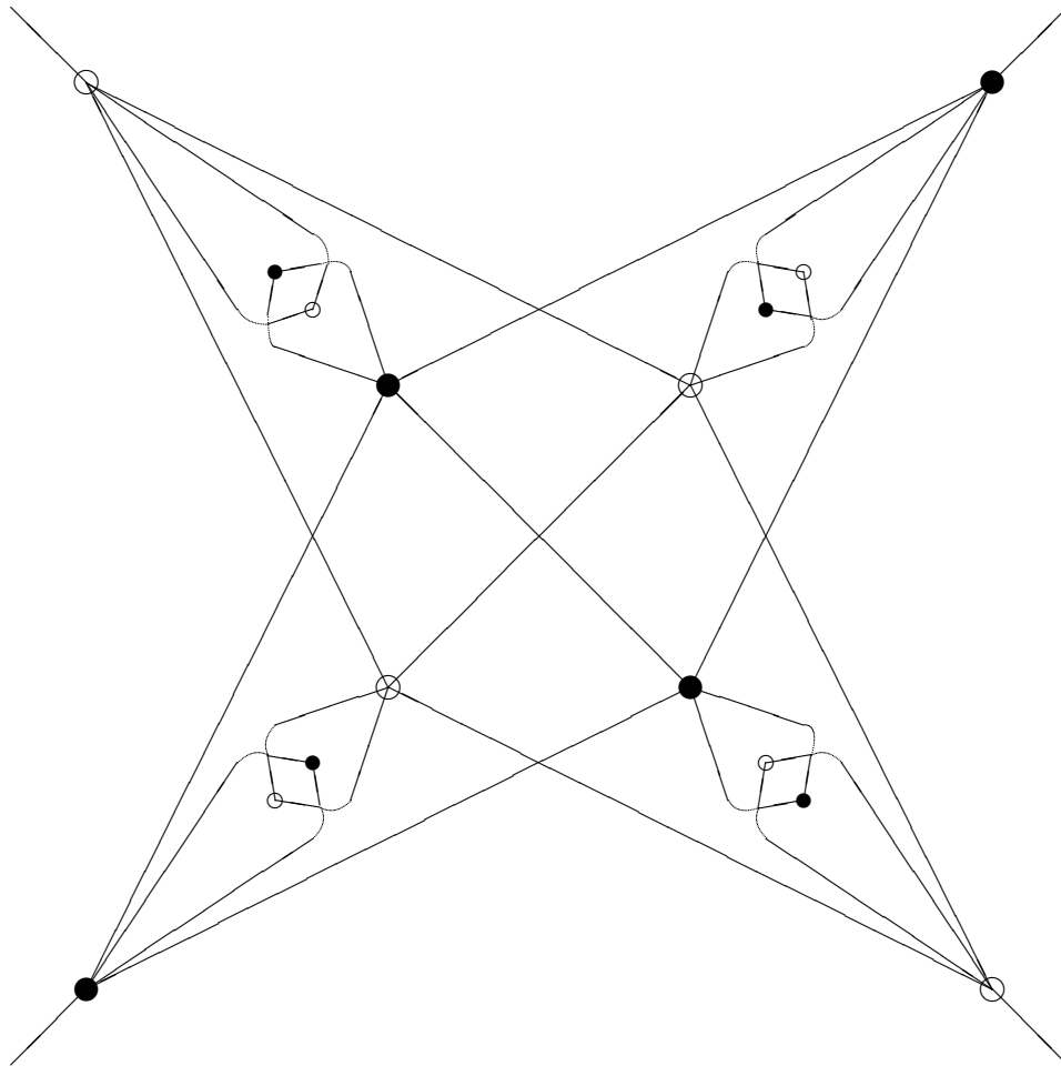
FIGURE 18. [2, 4] \triangleright [2^+, 4]
