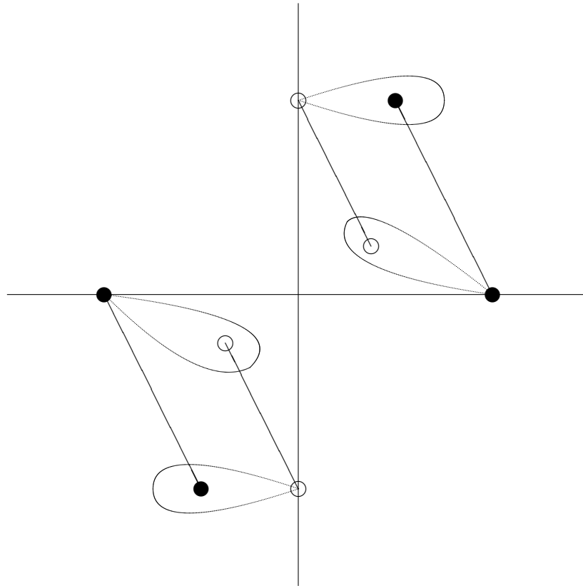
FIGURE 28. [2, 2^+] \triangleright [2^+, 2^+]
