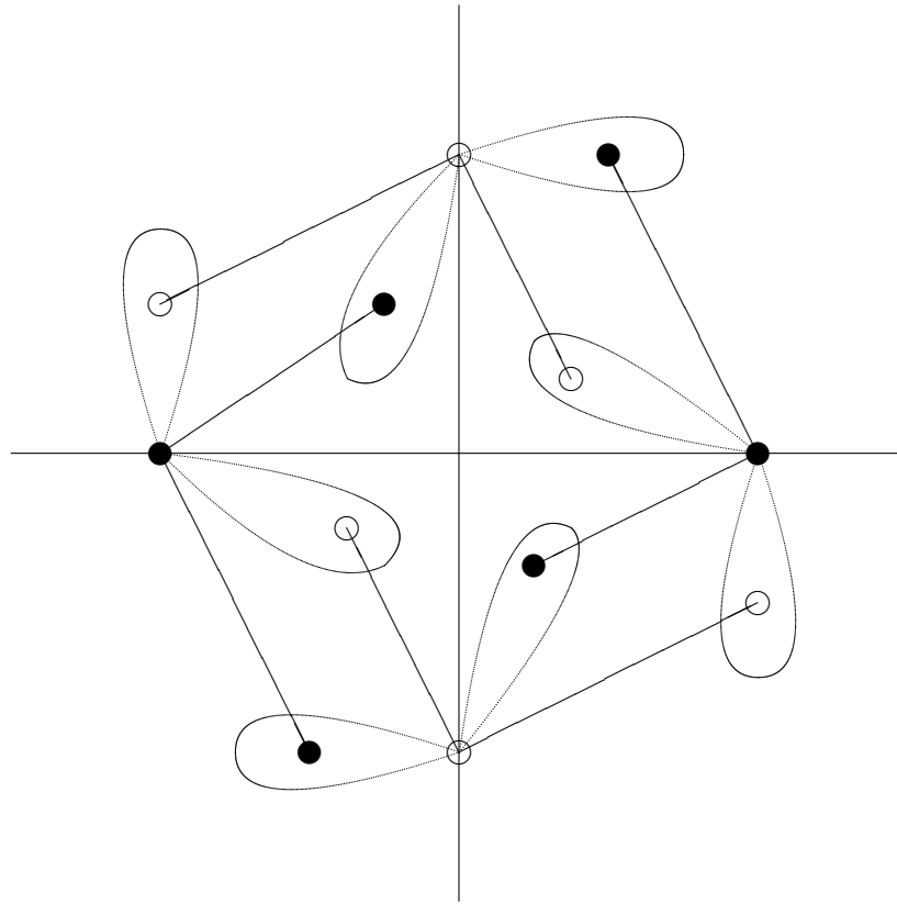
FIGURE 22. [2, 4]^+ \triangleright [2, 2]^+
