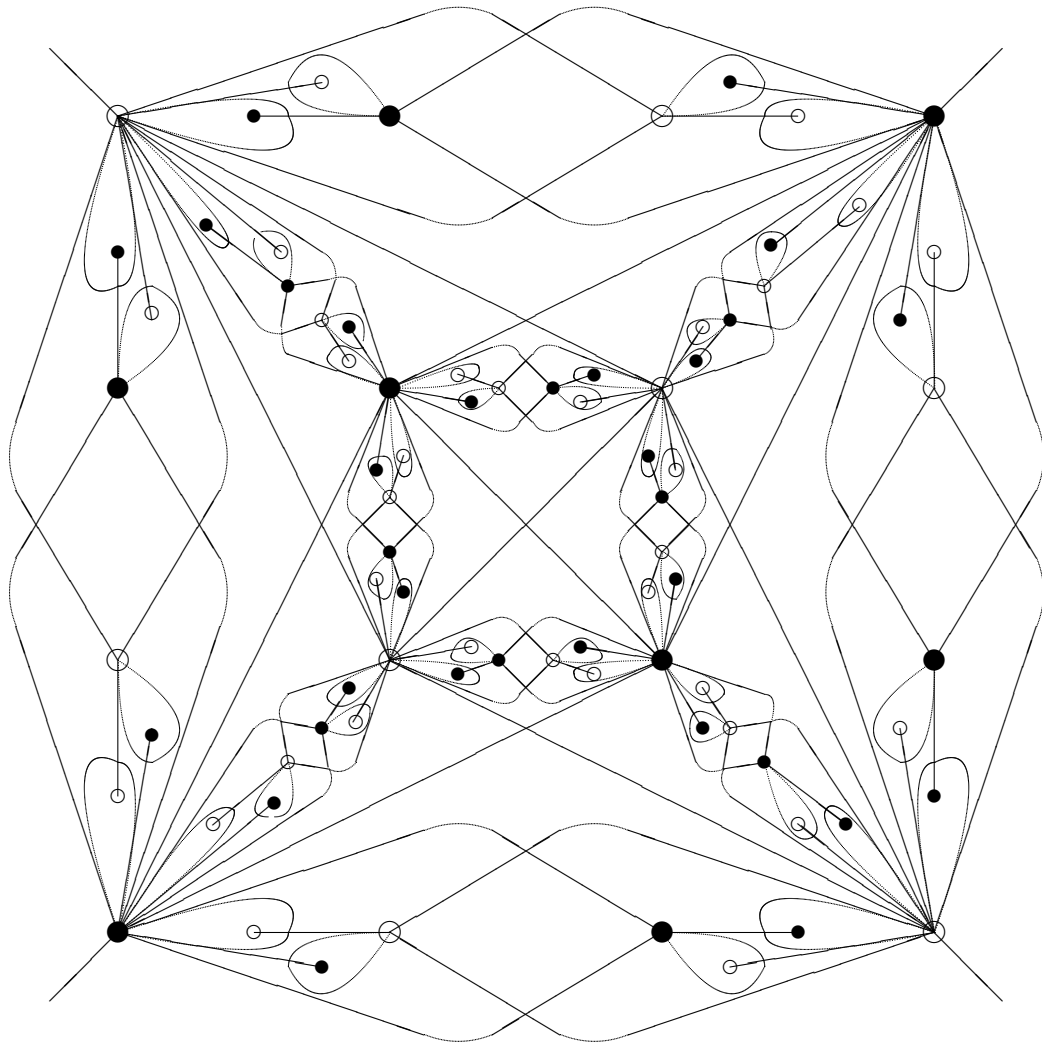
FIGURE 34. [3^+, 4] \triangleright [3, 3]^+
