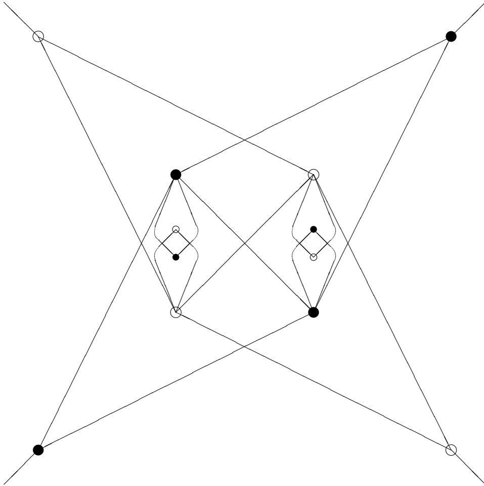
FIGURE 12. [2] \triangleright [2]^+
