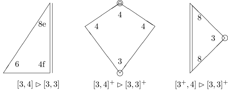
FIGURE 10. Pairings with \text{Dual}(G) acting on the cube
