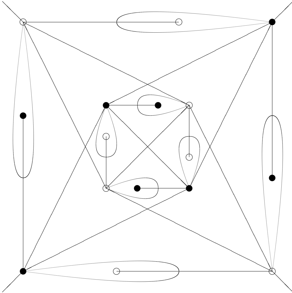
FIGURE 27. [2, 4^+] \triangleright [2^+, 4^+]
