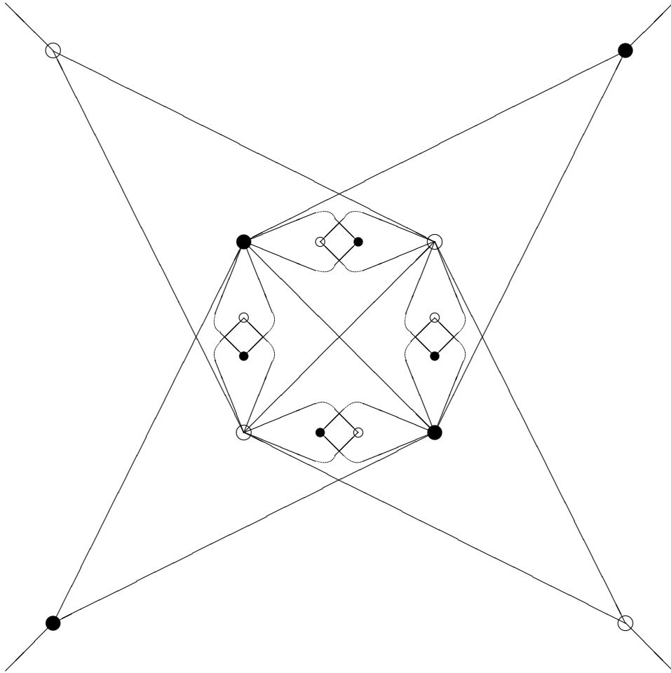
FIGURE 13. [4] \triangleright [2]
