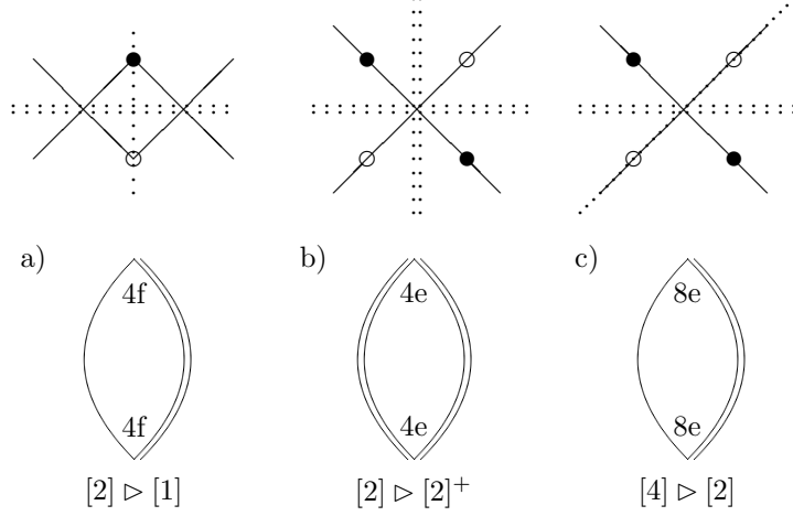
FIGURE 3. \text{Dual}(G) = [q]
