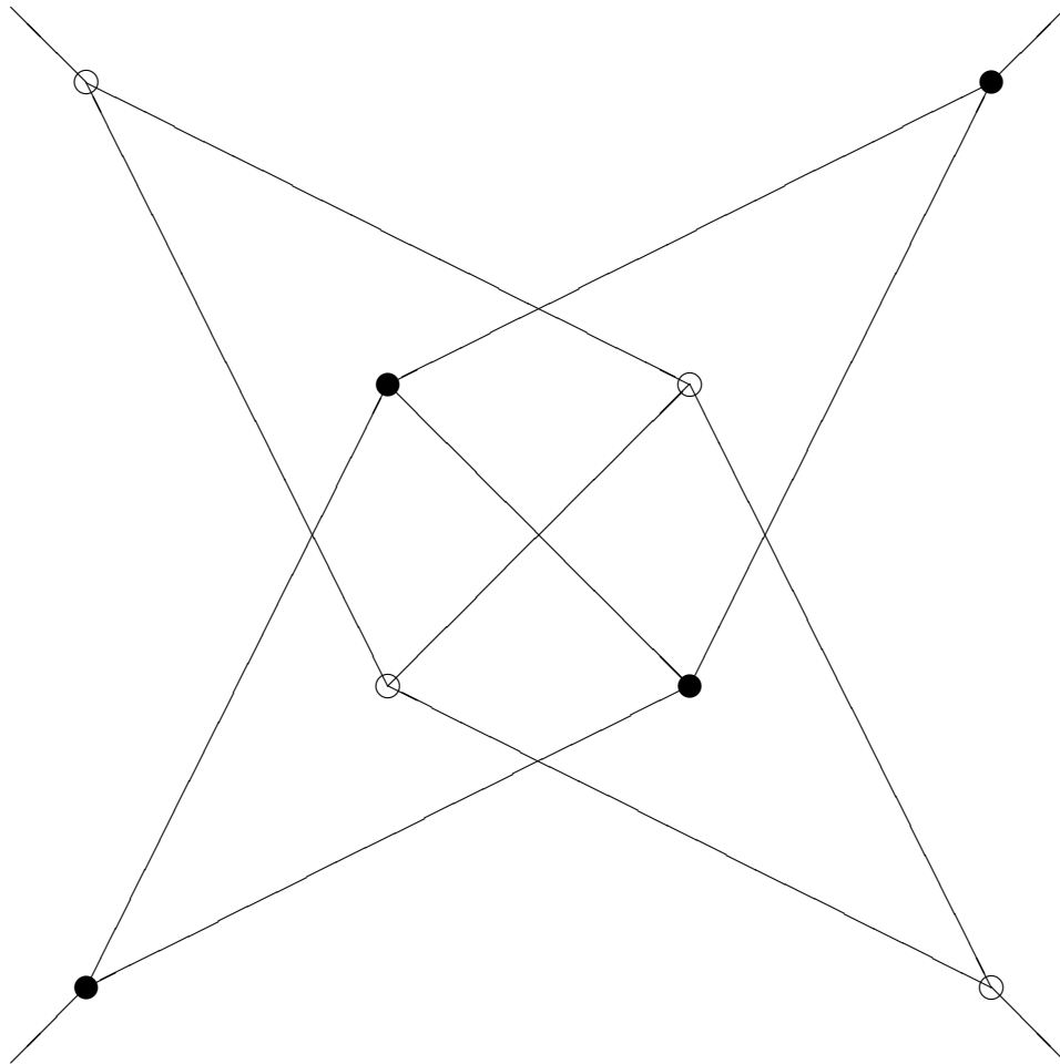
FIGURE 32. [3, 4] \triangleright [3, 3]
