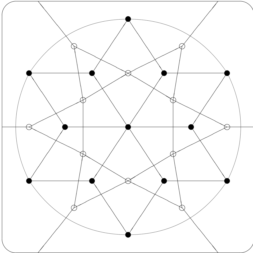
FIGURE 16. [2, 6] \triangleright [6]
