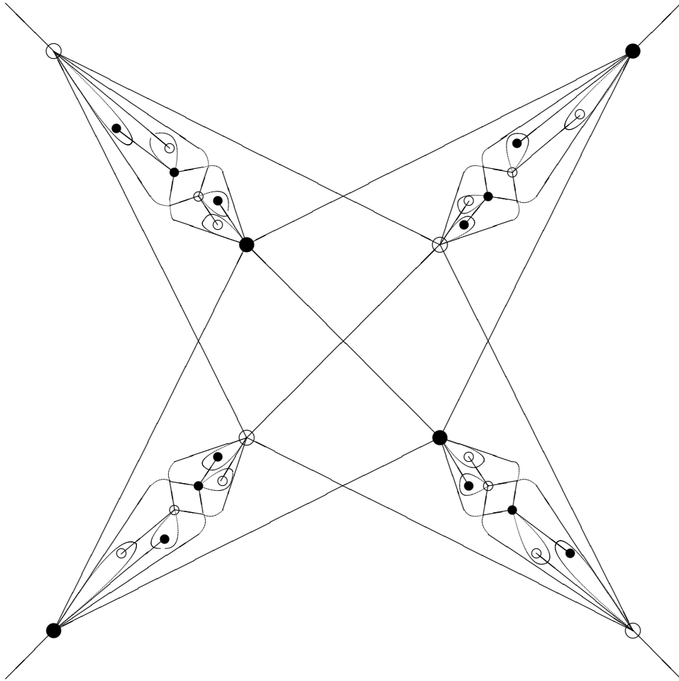
FIGURE 17. [2, 2] \triangleright [2, 2]^+
