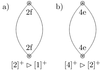
FIGURE 4. \text{Dual}(G) = [q]^+
