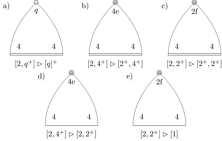
FIGURE 8. \text{Dual}(G) = [2, q^+]
