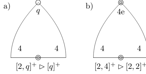
FIGURE 6. \text{Dual}(G) = [2, q]^+
