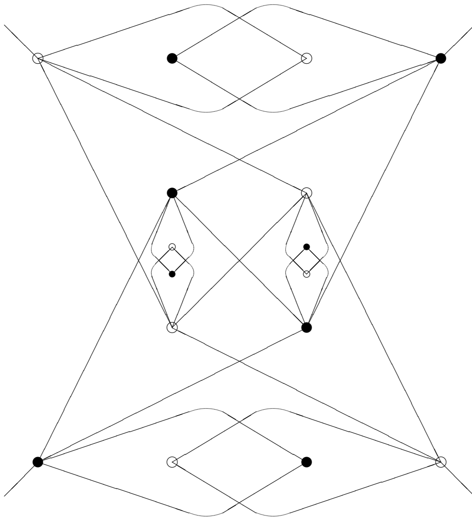
FIGURE 25. [2^+, 4] \triangleright [2^+, 4^+]
