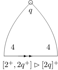
FIGURE 9. \text{Dual}(G) = [2^+, 2q^+]
