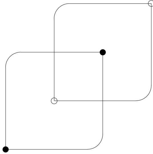
FIGURE 20. [2, 4] \triangleright [2, 2]
