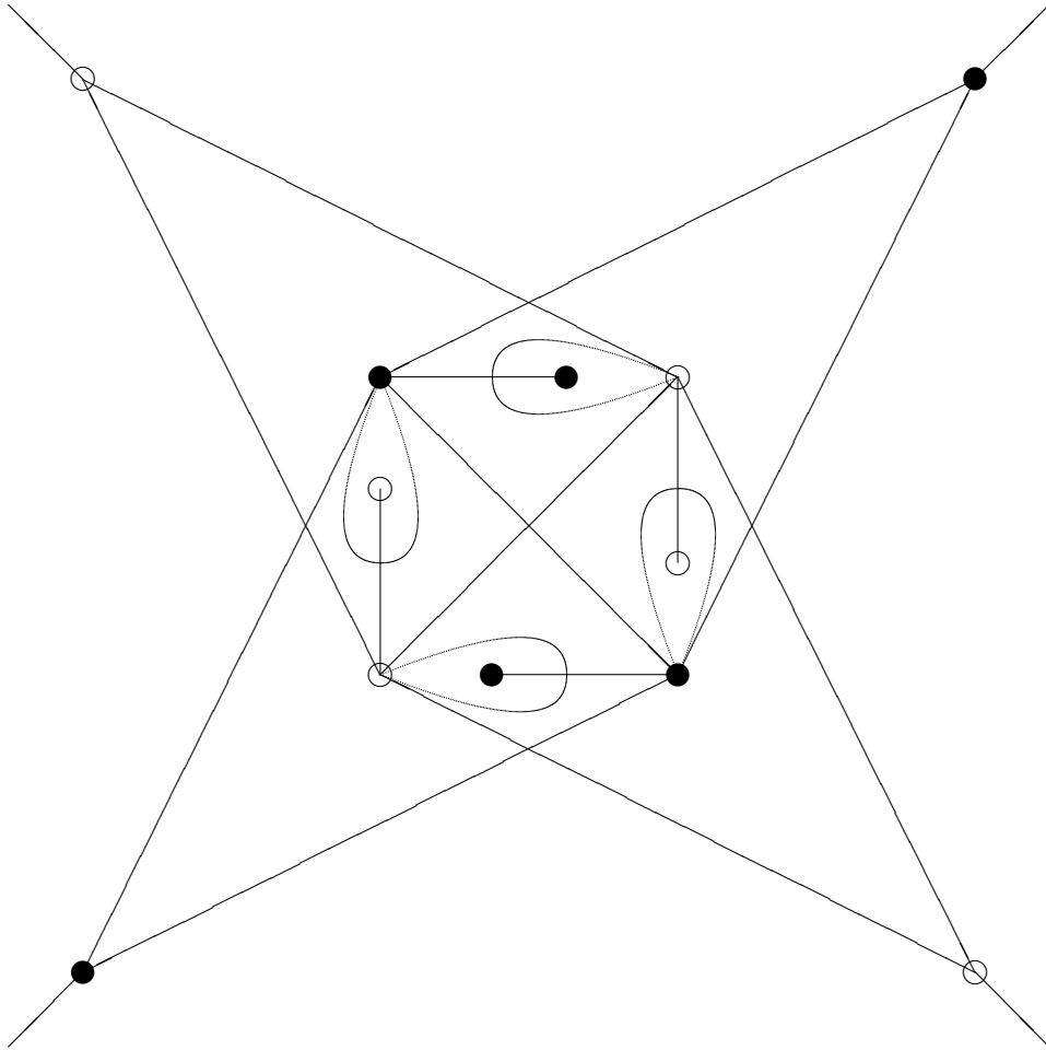
FIGURE 15. [4]^+ \triangleright [2]^+
