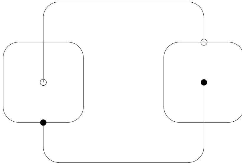
FIGURE 30. [2, 2^+] \triangleright [1]
