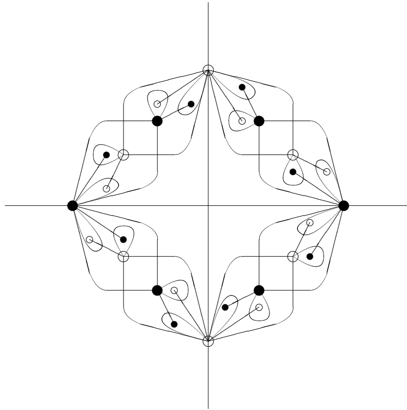
FIGURE 24. [2^+, 4] \triangleright [2, 2]^+
