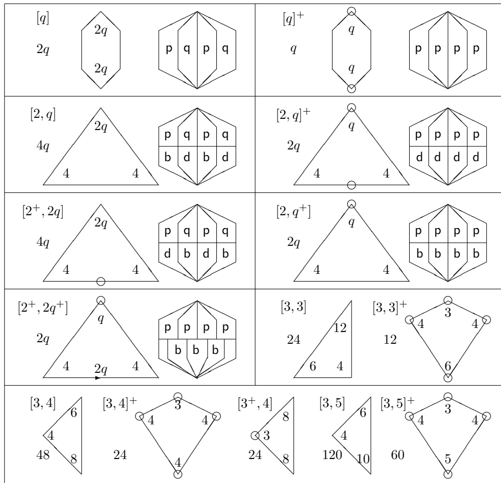
FIGURE 1. The finite groups of the sphere. The number below the group symbol is the order of the group, and the illustration on the right of the first seven panels indicates how the fundamental region, in which is drawn a “p”, is transformed by the group.
