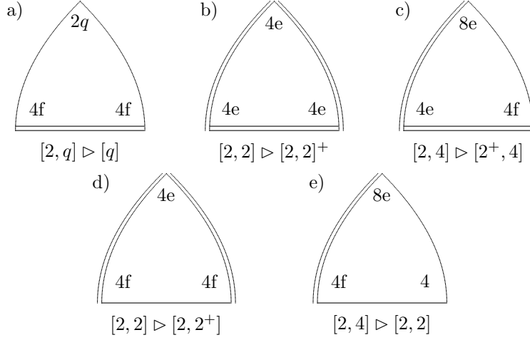
FIGURE 5. \text{Dual}(G) = [2, q]
