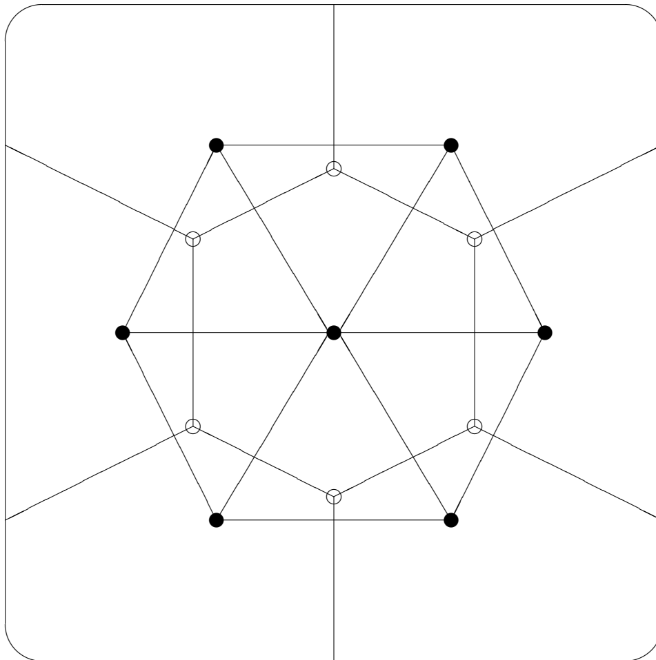
FIGURE 23. [2^+, 12] \triangleright [12]
