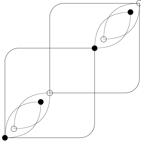
FIGURE 19. [2, 2] \triangleright [2, 2^+]
