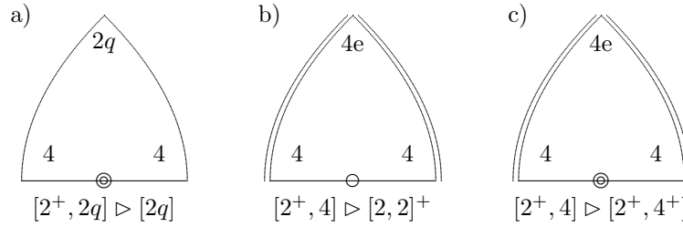
FIGURE 7. \text{Dual}(G) = [2^+, 2q]
