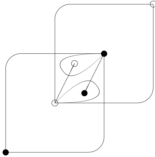
FIGURE 14. [2]^+ \triangleright [1]^+
