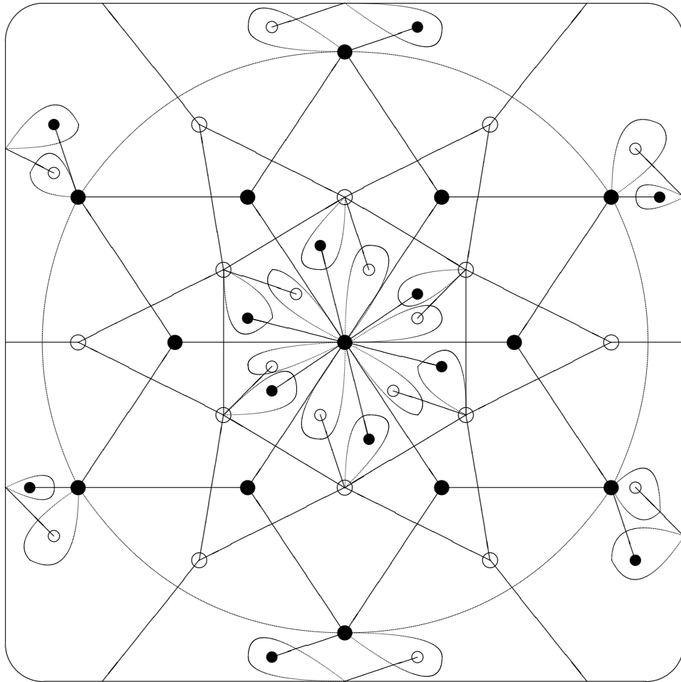
FIGURE 26. [2, 6^+] \triangleright [6]^+
