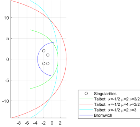
(a) Talbot's contours
