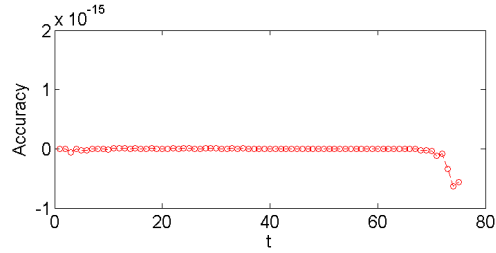
(b) Fixed Talbot method
