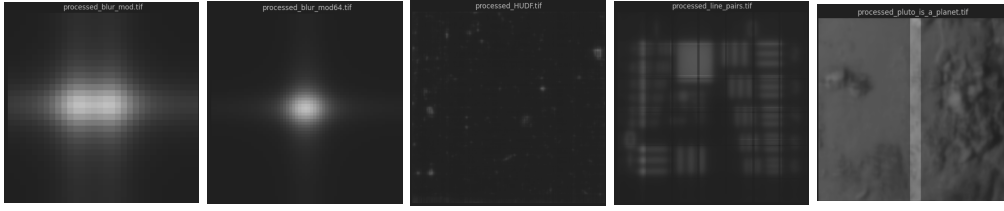
Figure 11. \alpha = \beta = \tau = 0.1 , \epsilon = 0.0001 . One iteration.
