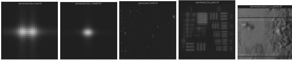
Figure 10. \alpha = \beta = \tau = 0.1, \epsilon = 0.001 . One iteration.
