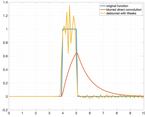
(a) De-blurring a single pulse
