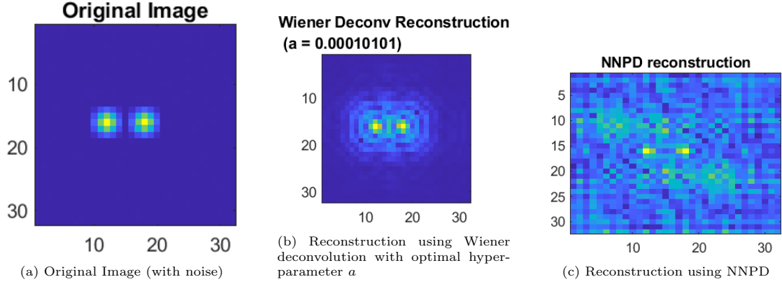
Figure 14. Comparison of different image reconstruction methods.
