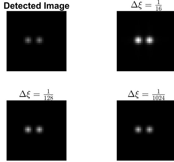
Figure 16. TGF with parameters a = b = 0.25 , c = 15
