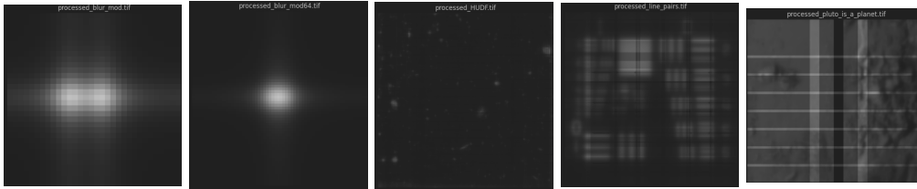
Figure 12. Reduced \alpha and \beta .
