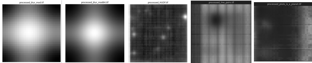
Figure 13. n=10 iterations. \alpha = \beta = 0.1
