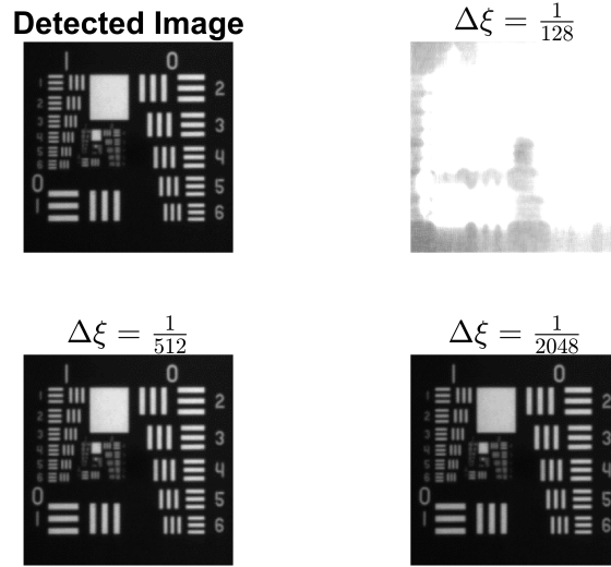
Figure 17. a = b = 0.5 , c = 15 , image size 246-by-245.
