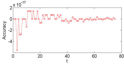
(a) Talbot method
