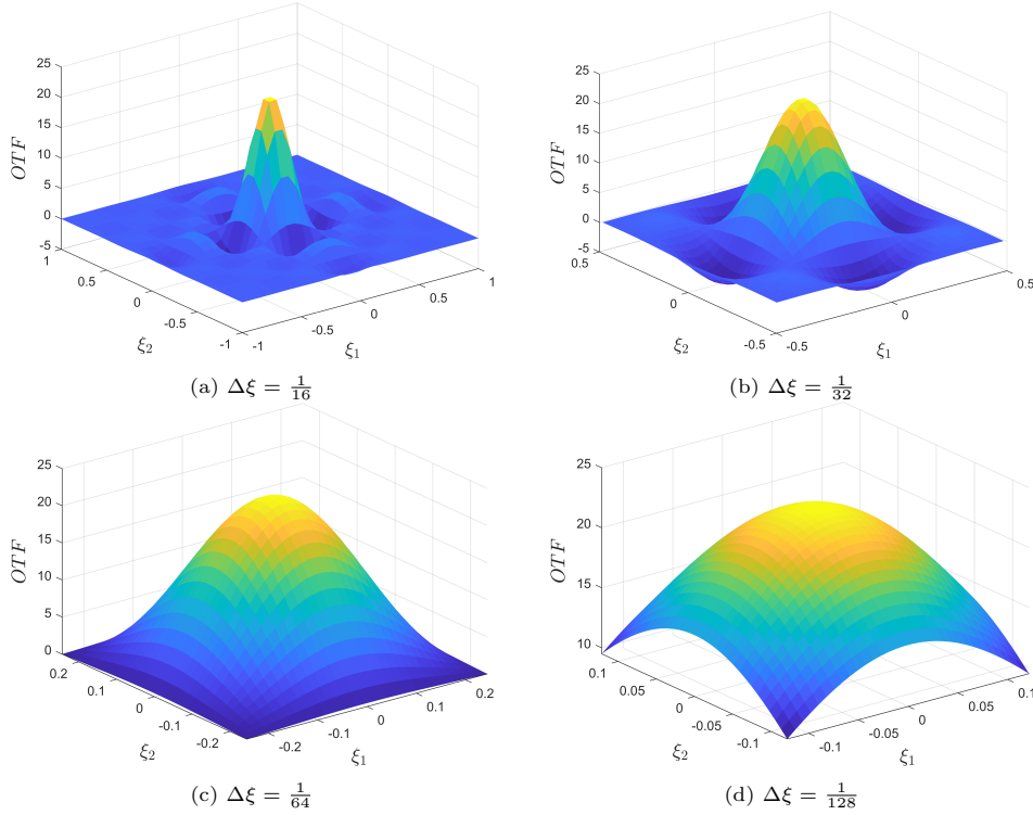
Figure 15. Truncated OTF per eq. 5.2b for an intended 32-by-32 image at various resolutions of the mesh grid: (a) \Delta\xi = \frac{1}{16} (b) \Delta\xi = \frac{1}{32} (c) \Delta\xi = \frac{1}{64} and (d) \Delta\xi = \frac{1}{128} . For all sample plots, Gaussian parameters per eq. 5.1 are fixed: a = b = 2 and c = 15 .
