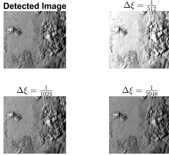
Figure 18. Same TGF parameters as Figure 17, image size 441-by-481.
