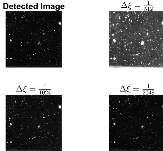
Figure 19. Same TGF parameters as Figure 17, image size 820-by-820.
