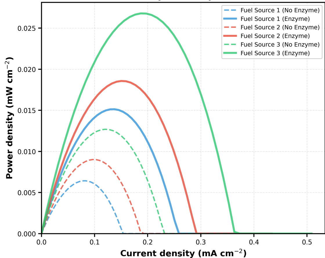
Power Density Curves by Fuel Source
