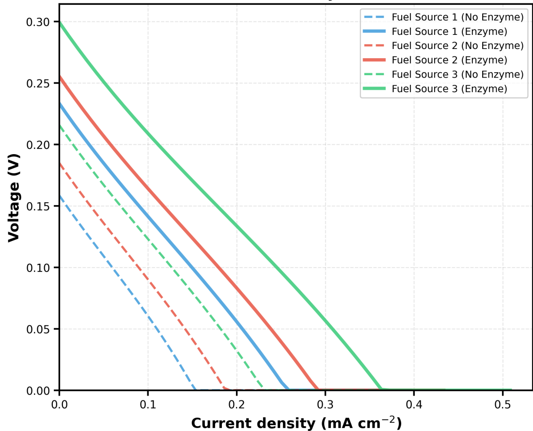
Polarization Curves by Fuel Source
