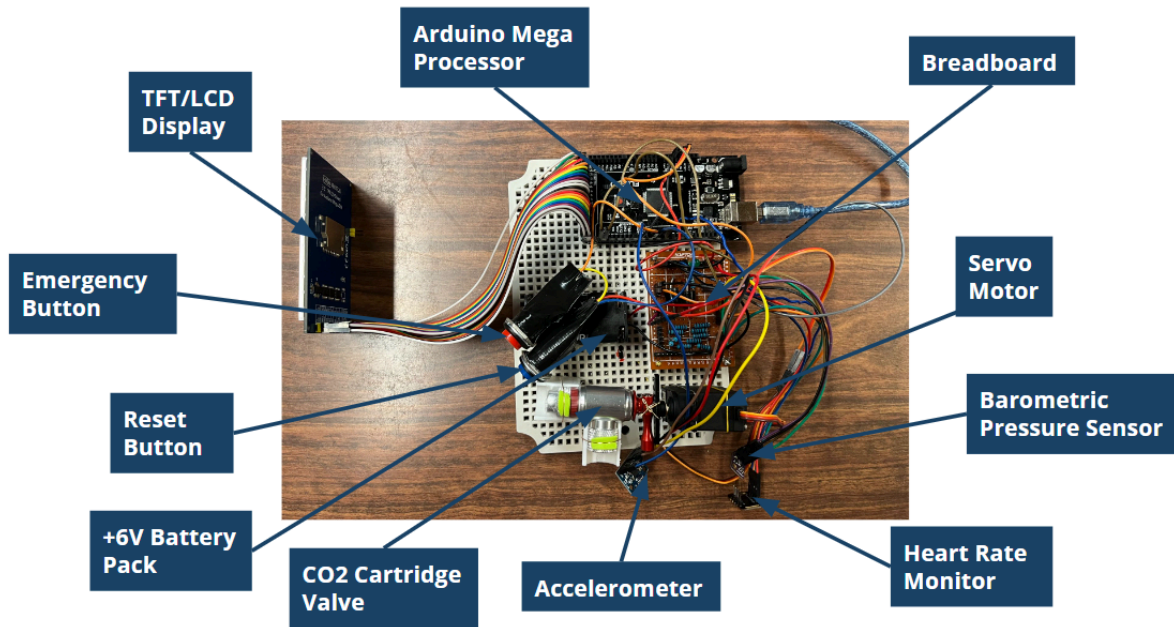
Figure 2: Diagram of the final prototype.
