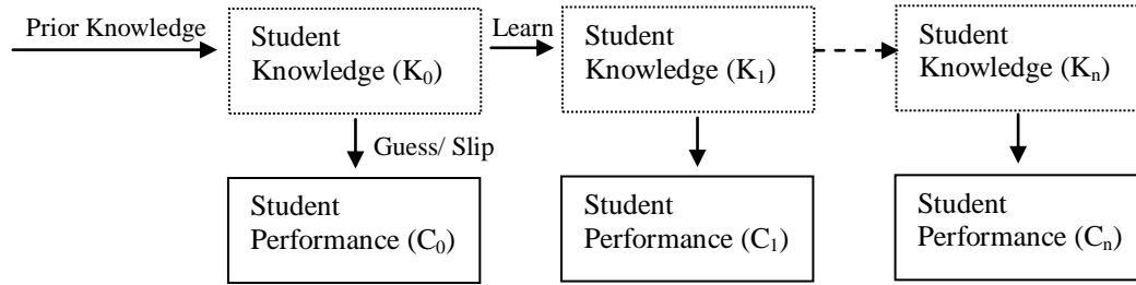
Figure 1 Knowledge tracing model
