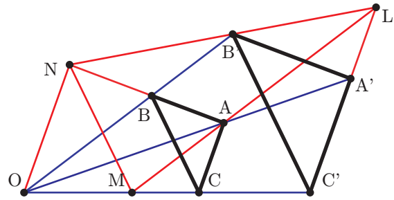
FIGURE 1. Using the Desargues Configuration.
